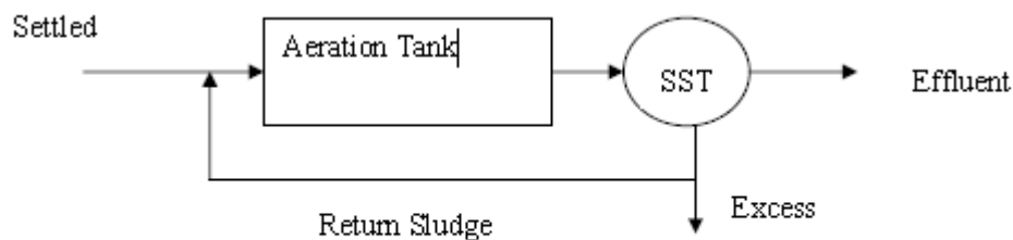
Figure 19.1 Conventional Activated Sludge Process
